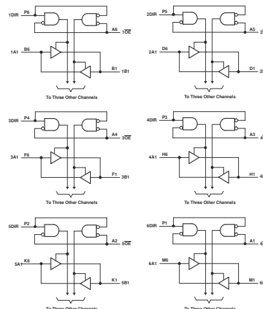
Figure 3-1. Logic Diagram
