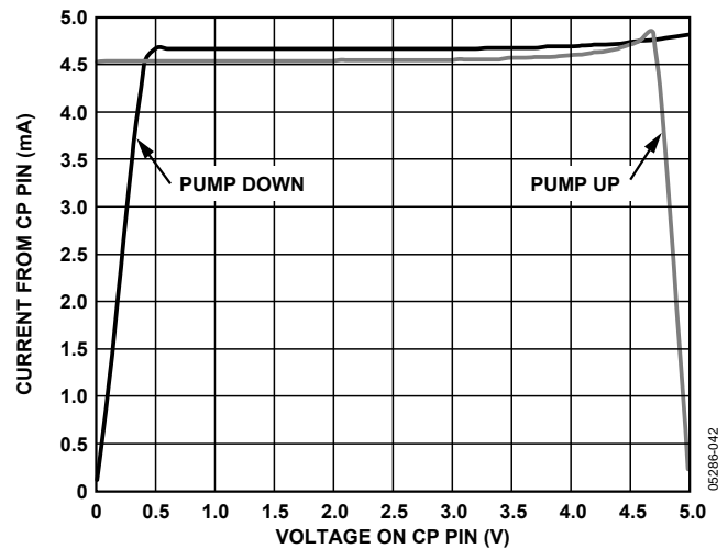
Figure 17. Charge Pump Output Characteristics @ V_{CP5} = 5.0\text{ V}
