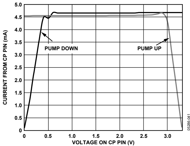
Figure 14. Charge Pump Output Characteristics @ V_{CP5} = 3.3\text{ V}
