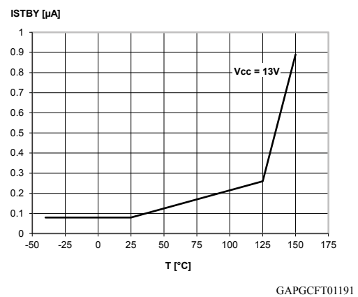
Figure 16. Standby current
