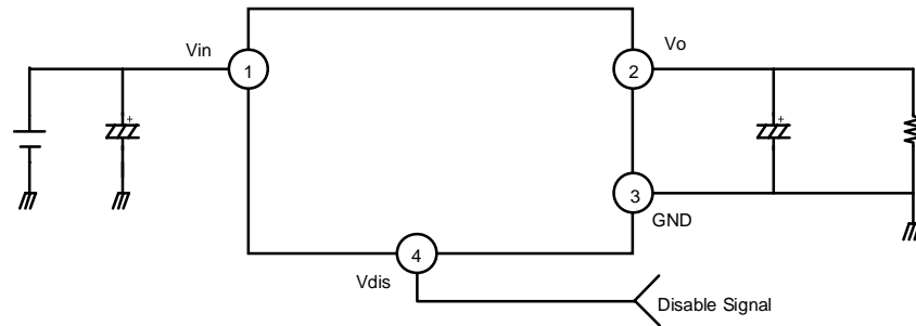
Figure 1. Application Circuit
