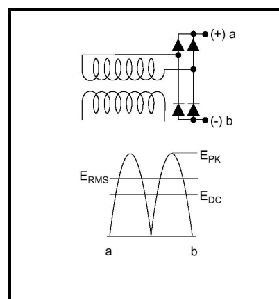
Fig. 3 : Full wave bridge
