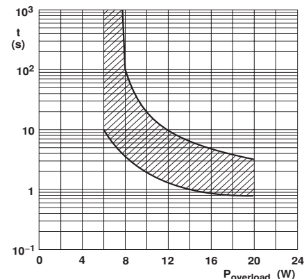
NFR25H This graph is based on measured data which may deviate according to the application. Fusing Characteristic.
