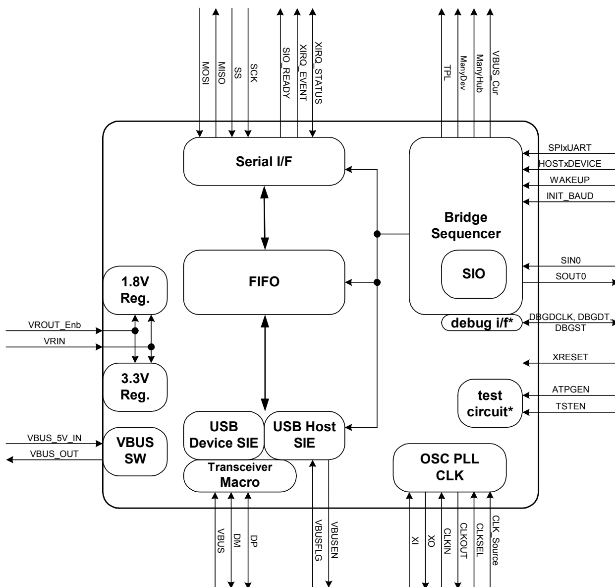
Fig. 3.1 Block diagram
