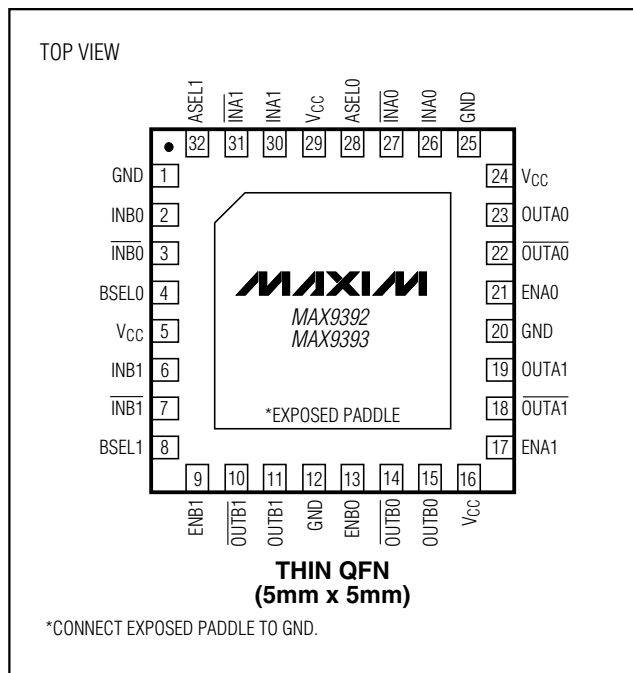
Pin Configurations (continued)
