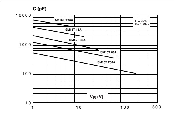
Figure 4. Capacitance versus reverse applied voltage for unidirectional types (typical values)
