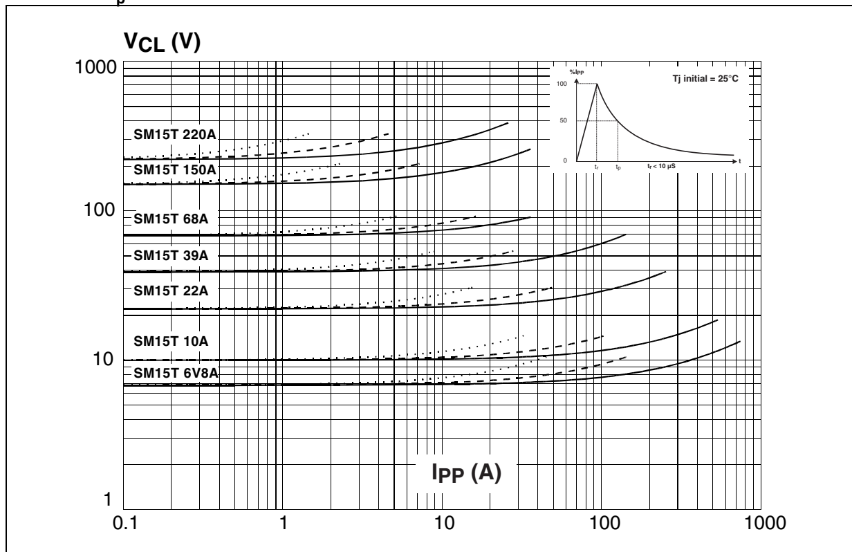
Figure 3. Clamping voltage versus peak pulse current Exponential waveform t p = 20 ms t p = 1 ms ————— t p = 10 ms.....
