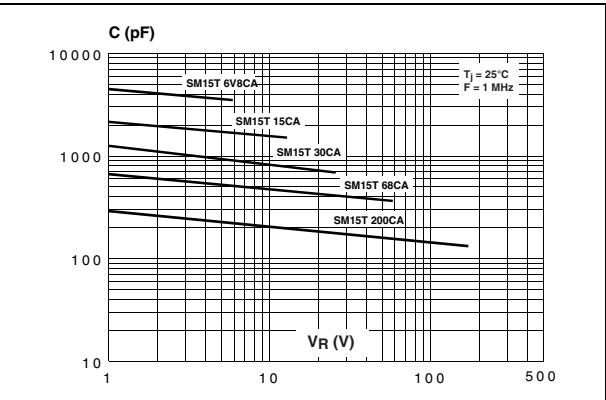
Figure 5. Capacitance versus reverse applied voltage for bidirectional types (typical values)
