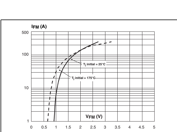
Figure 6. Peak forward voltage drop versus peak forward current (typical values for unidirectional types)
