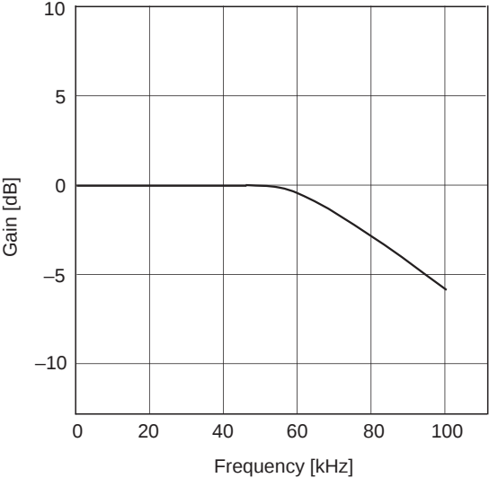
Stereo LPF frequency response
