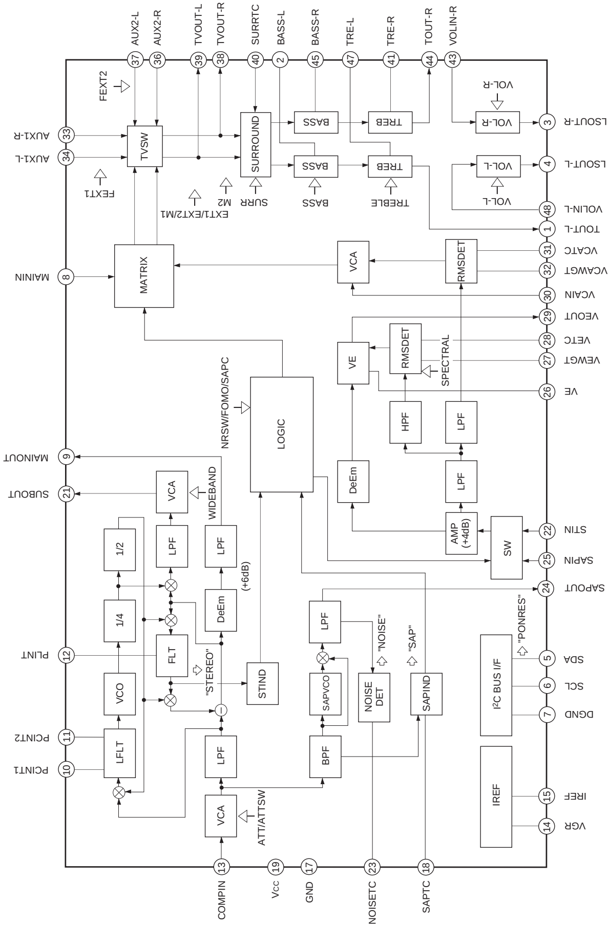
Block Diagram
