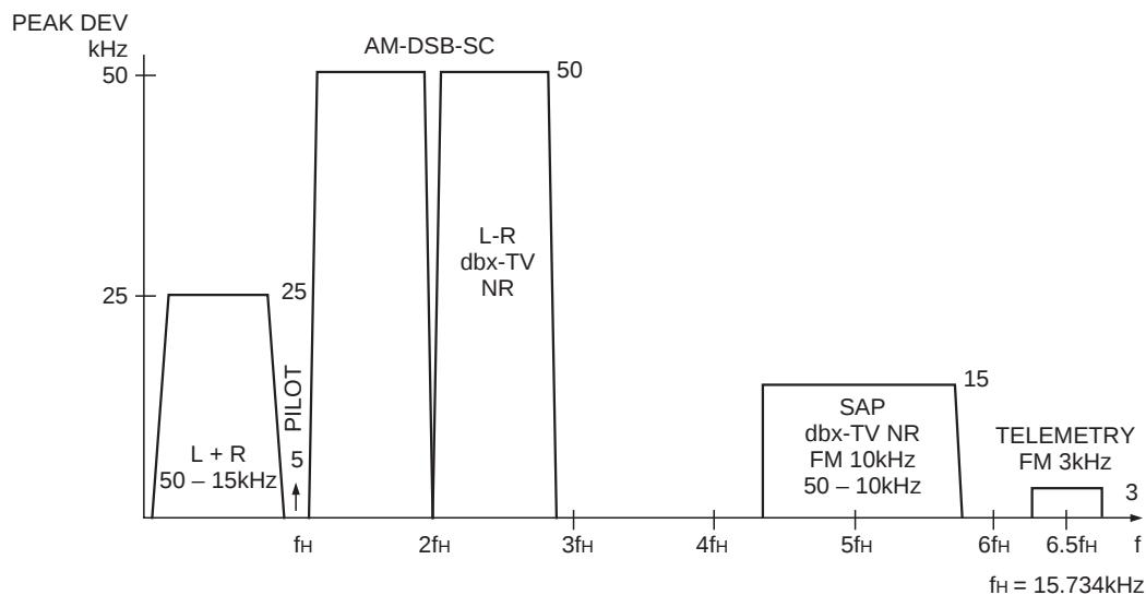
Fig. 1. Base-band spectrum
