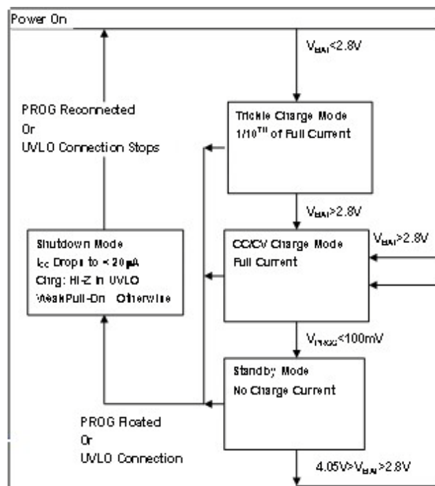
Figure1. State Diagram of a Typical Charge Cycle
