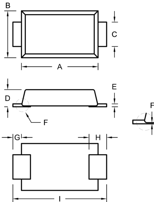
Thin SMA
