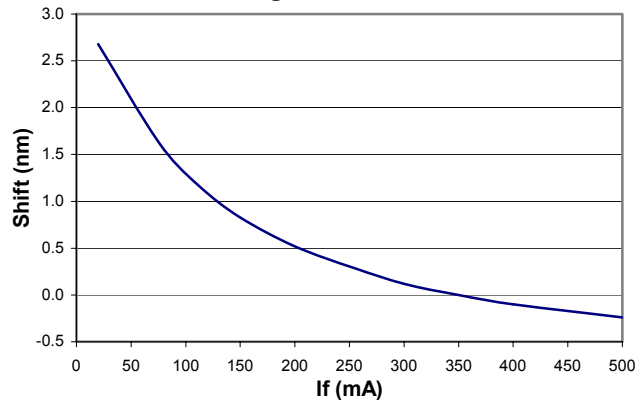
Dominant Wavelength Shift vs Forward Current
