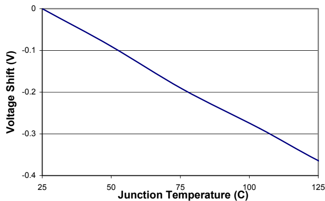
Voltage Shift vs Junction Temperature
