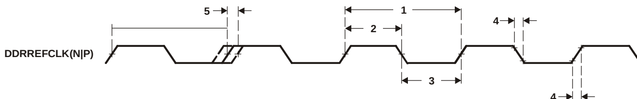
Figure 8-15 DDRREFCLK(N|P) Timing
