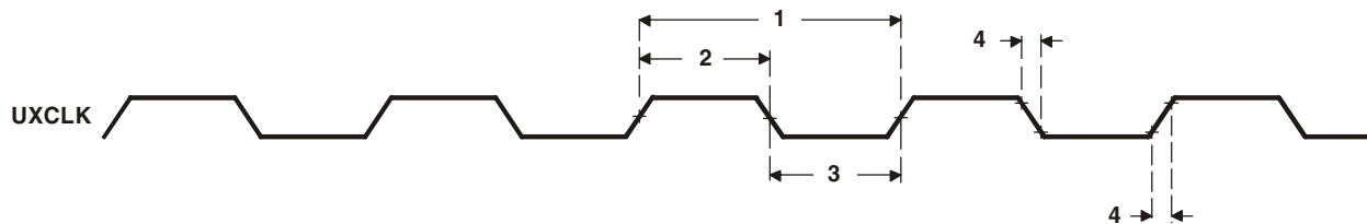
Figure 8-46 UXCLK Timing
