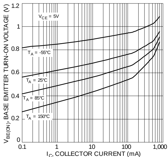
Figure 4 Typical Base Emitter Turn-On Voltage vs. Collector Current
