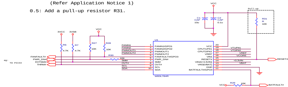
SMARTFAN1 Speed Control Circuit
