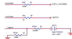
VOLTAGE SENSING CIRCUIT
