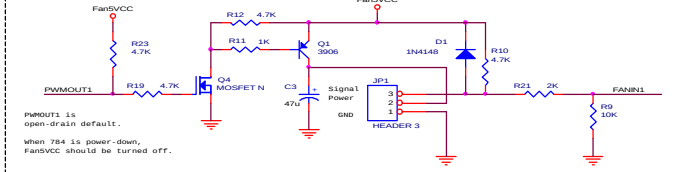
SMARTFAN1 Speed Control Circuit
