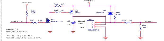
SMARTFAN2 Speed Control Circuit
