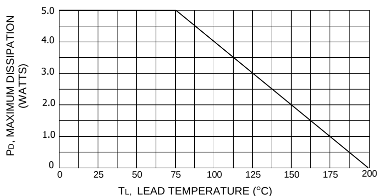
Fig. 1 POWER DERATING CURVE
