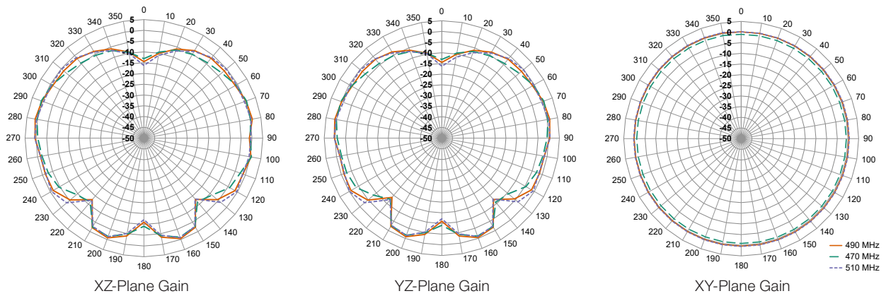
Figure 8. Radiation Patterns for CW 490 MHz Antenna
