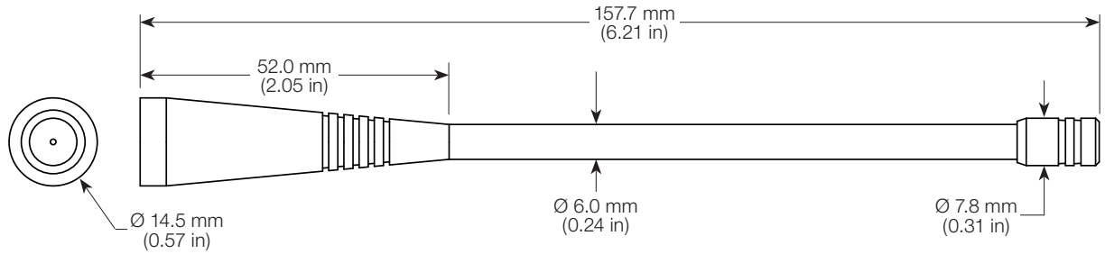
Figure 6. CW 490 MHz Antenna Dimensions
