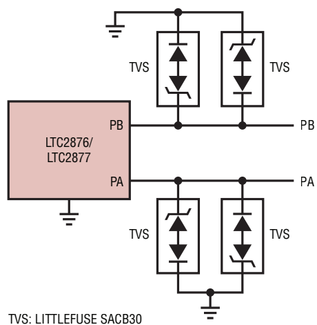
Figure 21. Exceptionally Robust, Low-Capacitance, ±30V Tolerant, ±4kV IEC 61000 Bus Protection Against Surge, EFT, and ESD. (See Auxiliary Protection for Surge, EFT, and ESD in the Applications Information Section for More Details)
