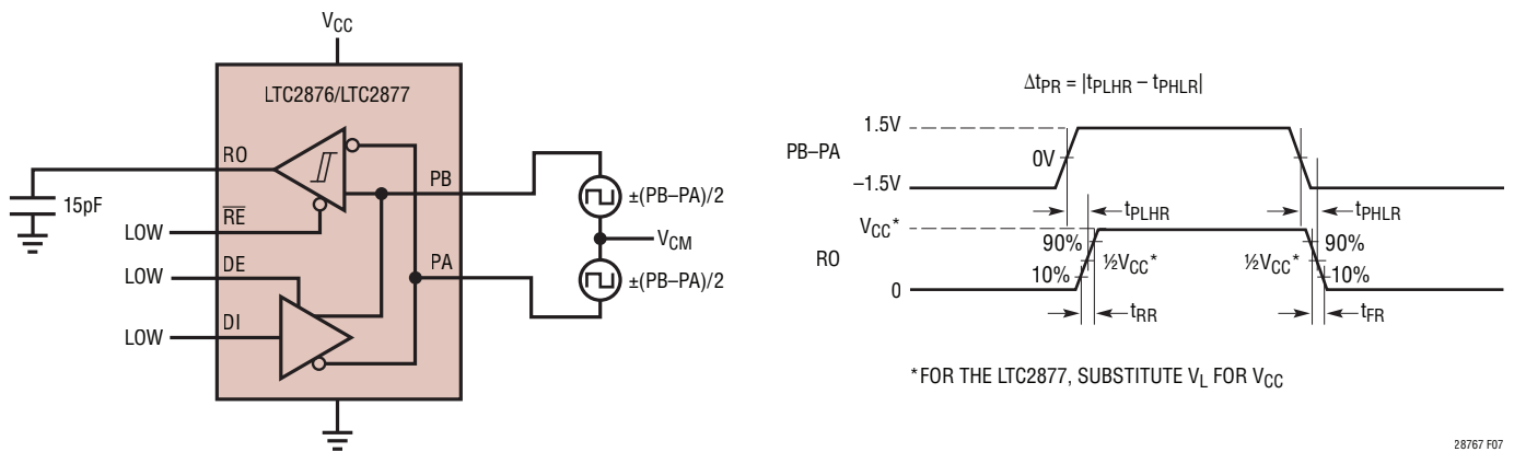
Figure 7. Receiver Propagation Delay Measurements
