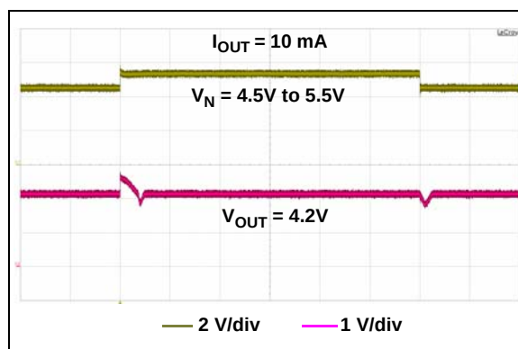
FIGURE 2-18: Dynamic Line Step ( V_R = 4.2\text{V} ).
