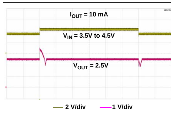
FIGURE 2-17: Dynamic Line Step ( V_R = 2.5\text{V} ).
