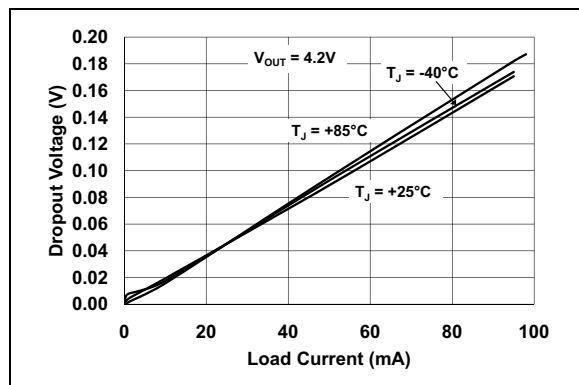
FIGURE 2-8: Dropout Voltage vs. Load Current ( V_R = 4.2\text{V} ).
