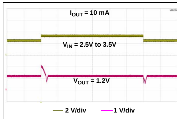
FIGURE 2-16: Dynamic Line Step ( V_R = 1.2\text{V} ).
