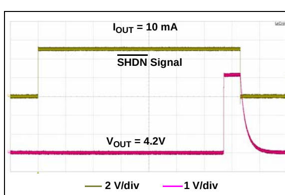
FIGURE 2-24: Startup From SHDN ( V_R = 4.2\text{V} ).
