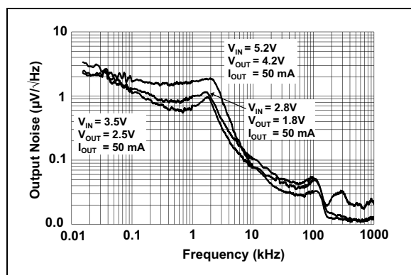
FIGURE 2-9: Noise vs. Frequency.
