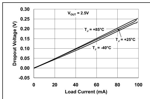
FIGURE 2-7: Dropout Voltage vs. Load Current ( V_R = 2.5\text{V} ).
