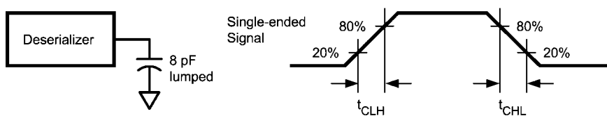
FIGURE 11. Deserializer LVCMOS/LVTTL Output Load and Transition Times
