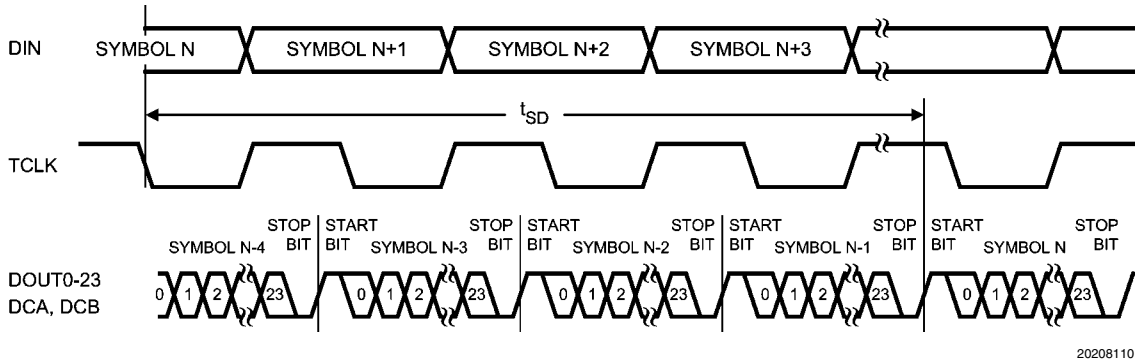
FIGURE 8. Serializer Delay
