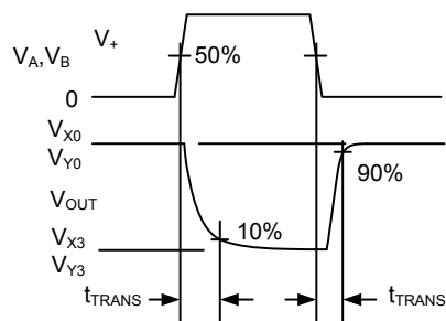
Test Circuit 3. Address Transition Times ( t_{TRANS} )
