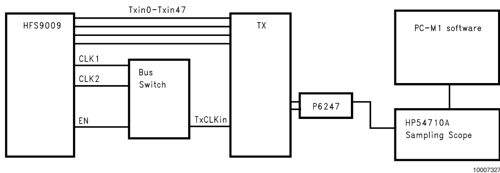
FIGURE 14. TJCC Test Setup - DS90C387
