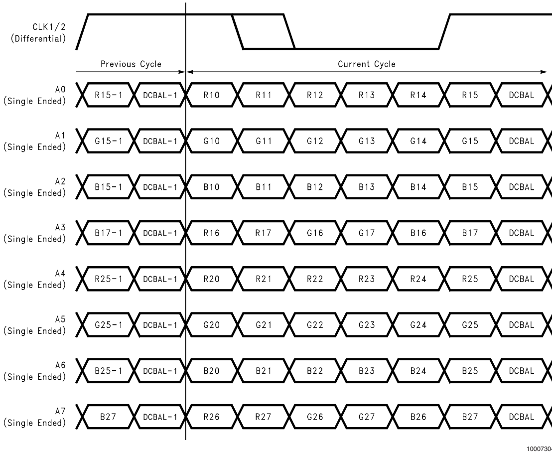
FIGURE 18. 48 Parallel TTL Data Inputs Mapped to LVDS Outputs DC Balanced Mode - Data Enabled, BAL=High
