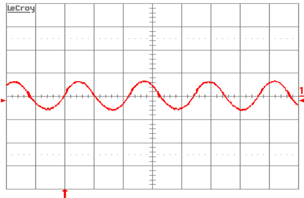
Figure 13: Input reflected ripple-current, i_c (200 mA/div.), through 10 measured at input terminals at full rated load current and V_{in} = 48\text{ V} . Refer to Figure 11 for test setup. Time scale: 1\ \mu\text{s}/\text{div} .
