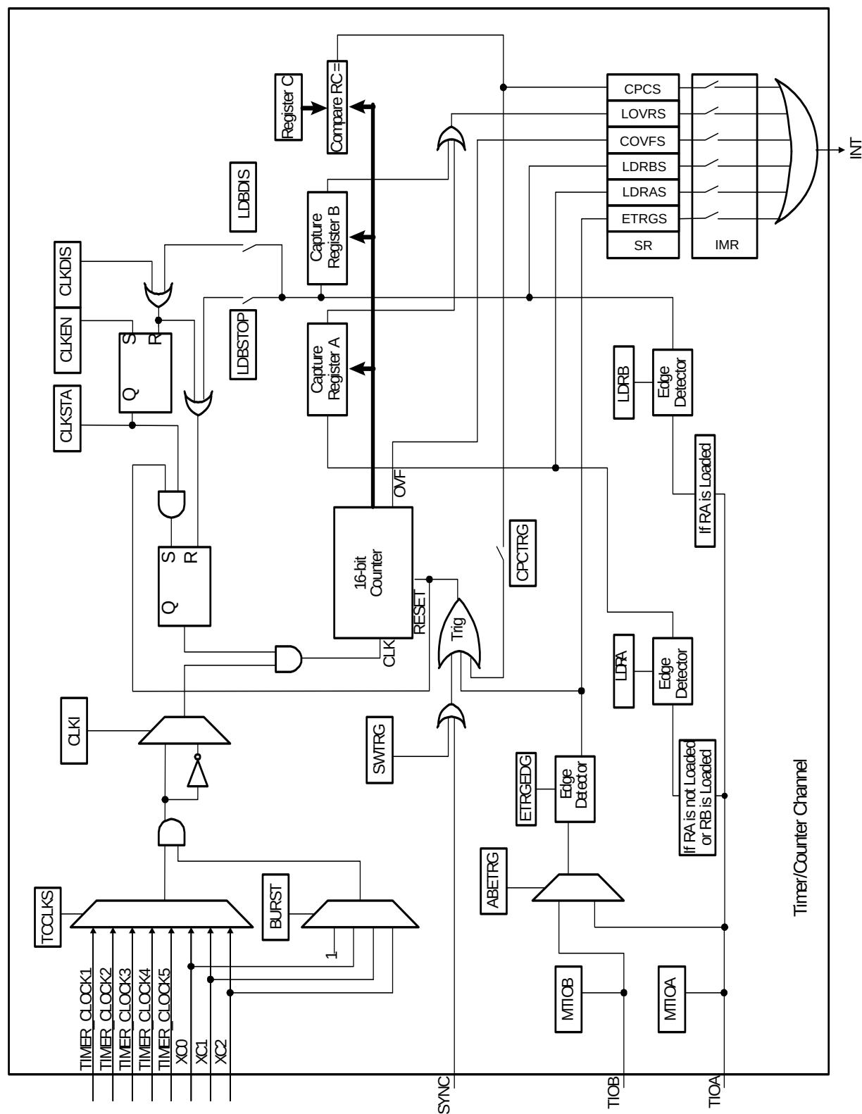
Figure 24-4. Capture Mode
