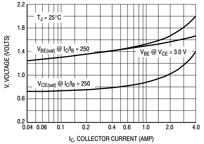
Figure 9. "On" Voltages
