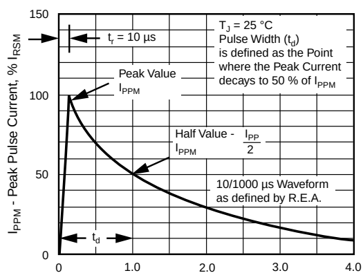
Fig. 3 - Pulse Waveform
