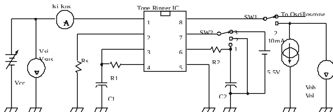
FIG. 4 Test Circuit (1)
