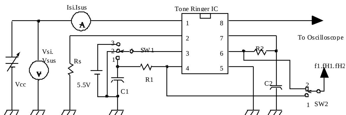
FIG. 4 Test Circuit (2)
