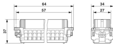
Female insert
