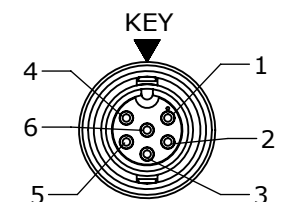
FACE VIEW P/N: CA62806PXXX90
