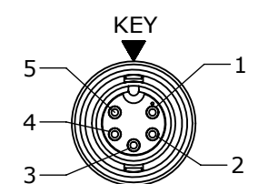
FACE VIEW P/N: CA62805PXXX90
