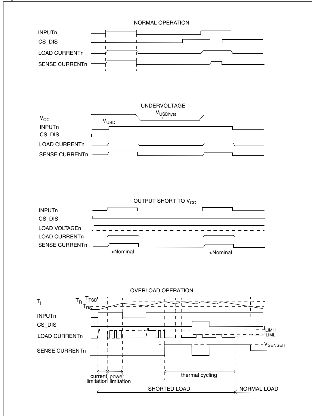
Figure 6. Waveforms
