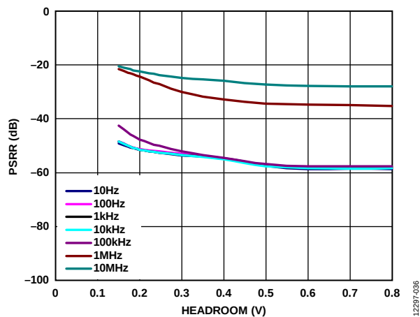
Figure 36. Power Supply Rejection Ratio (PSRR) vs. Headroom, V_{OUT} = 5\text{ V} , 500 mA Load Current, Different Frequencies
