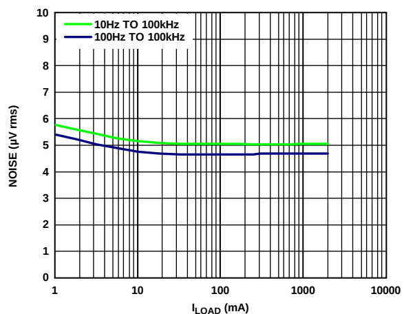
Figure 41. RMS Output Noise vs. Load Current ( I_{LOAD} ), V_{OUT} = 3\text{ V}
