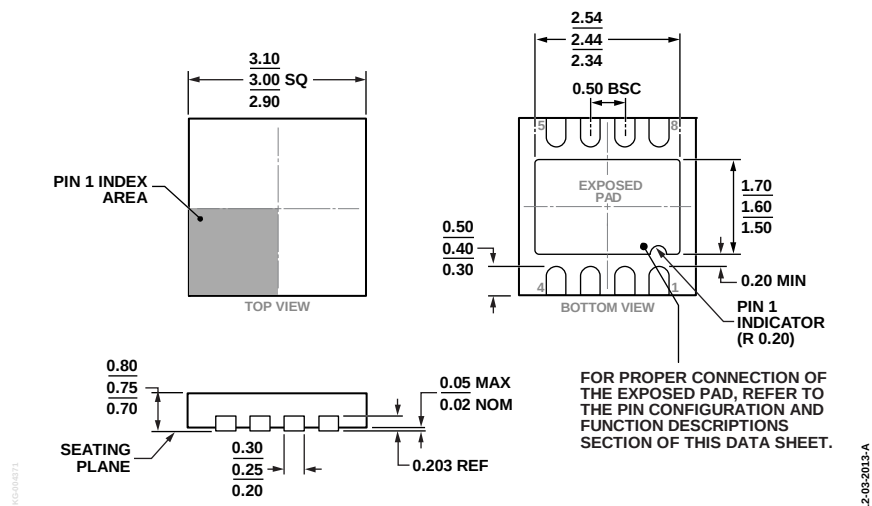
Figure 70. 8-Lead Lead Frame Chip Scale Package [LFCSP_WD] 3 mm × 3 mm Body, Very Very Thin, Dual Lead (CP-8-21) Dimensions shown in millimeters
