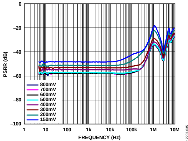
Figure 35. Power Supply Rejection Ratio (PSRR) vs. Frequency, V_{OUT} = 5\text{ V} , 500 mA Load Current, Various Headroom Voltages
