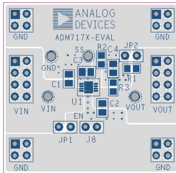
Figure 69. Example LFCSP PCB Layout
