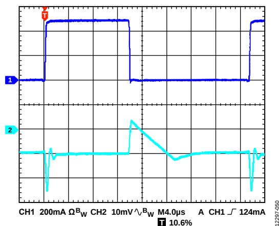
Figure 50. Load Transient Response, I_{LOAD} = 10\text{ mA} to 510\text{ mA} , Adjustable Version, V_{OUT} = 1.2\text{ V} , V_{IN} = 2.5\text{ V} , CH1 = I_{LOAD} , CH2 = V_{OUT}
