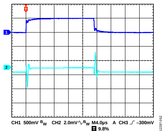
Figure 52. Line Transient Response, 6 V to 6.5 V, I_{LOAD} = 500 mA, V_{OUT} = 5 V, CH1 = V_{IN} , CH2 = V_{OUT}
