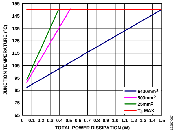
Figure 65. LFCSP, T A = 85°C
