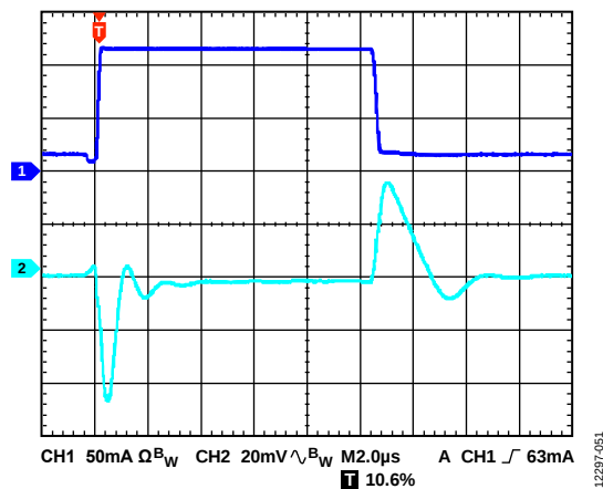
Figure 51. Load Transient Response, I_{LOAD} = 10\text{ mA} to 110\text{ mA} , Adjustable Version, V_{OUT} = 1.2\text{ V} , V_{IN} = 2.5\text{ V} , CH1 = I_{LOAD} , CH2 = V_{OUT}
