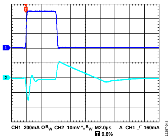
Figure 48. Load Transient Response, I_{LOAD} = 10\text{ mA} to 510\text{ mA} , V_{OUT} = 5\text{ V} , V_{IN} = 5.5\text{ V} , CH1 = I_{LOAD} , CH2 = V_{OUT}
