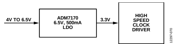
Figure 67. Clock Driver
