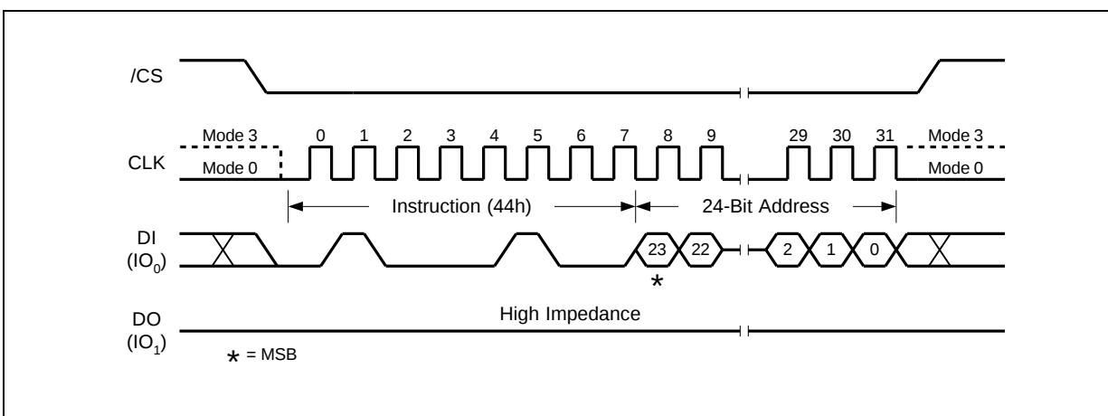
Figure 49. Erase Security Registers Instruction
