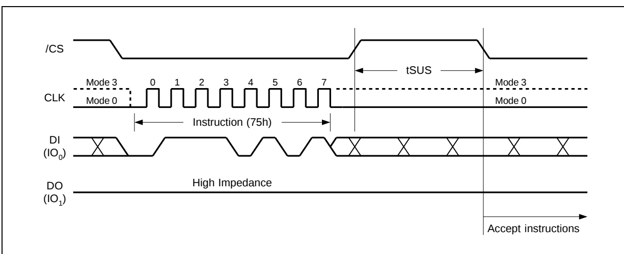
Figure 40. Erase/Program Suspend Instruction
