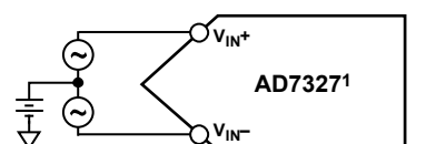
Figure 34. True Differential Inputs
