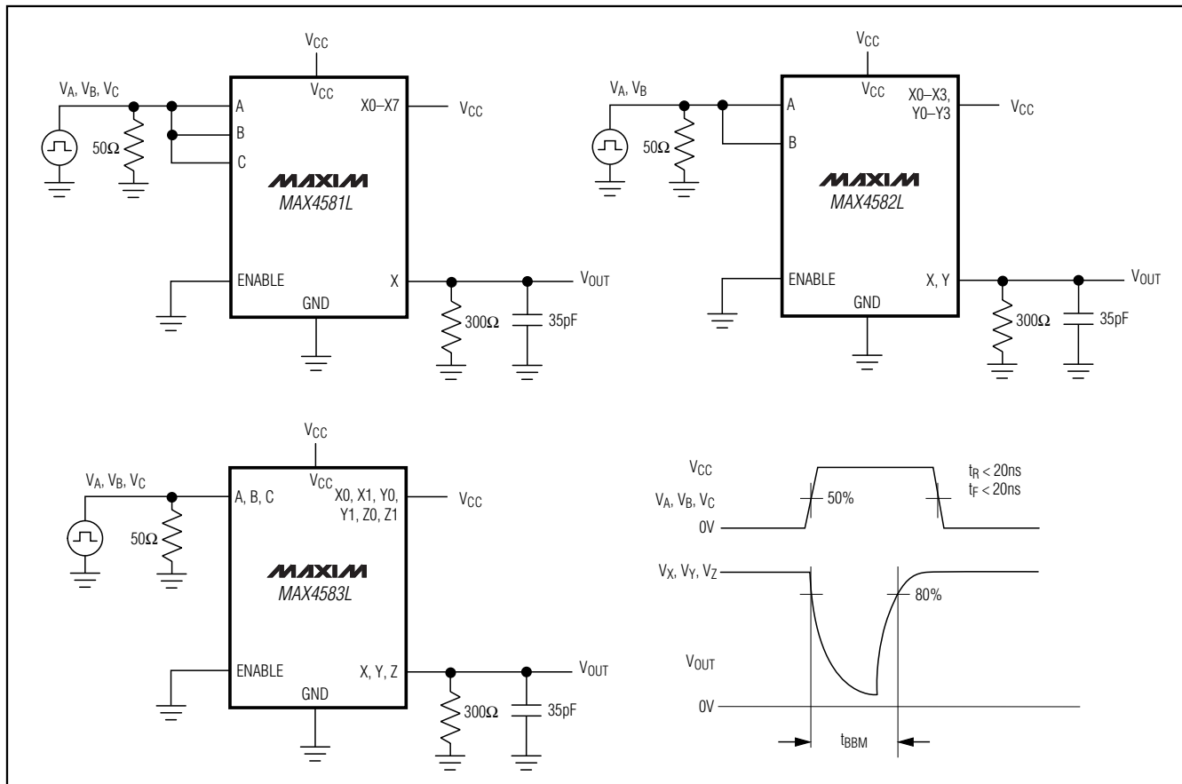
Figure 3. Break-Before-Make Interval
