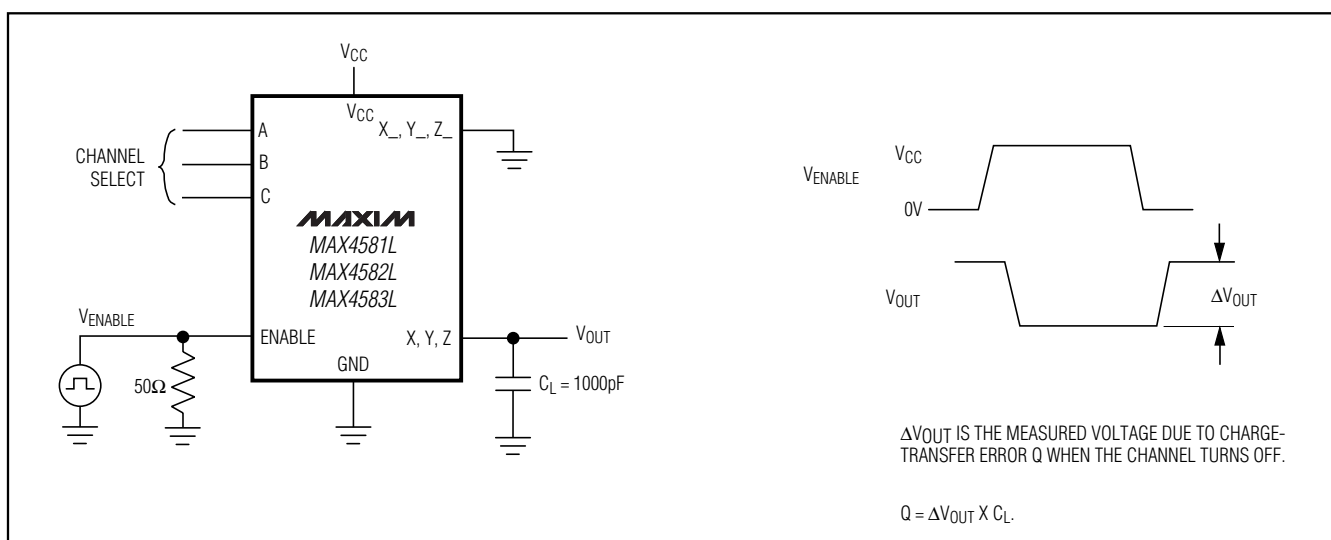
Figure 4. Charge Injection
