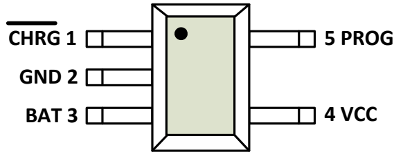
Figure 2 Pin Configuration of TD9054(Top View)
