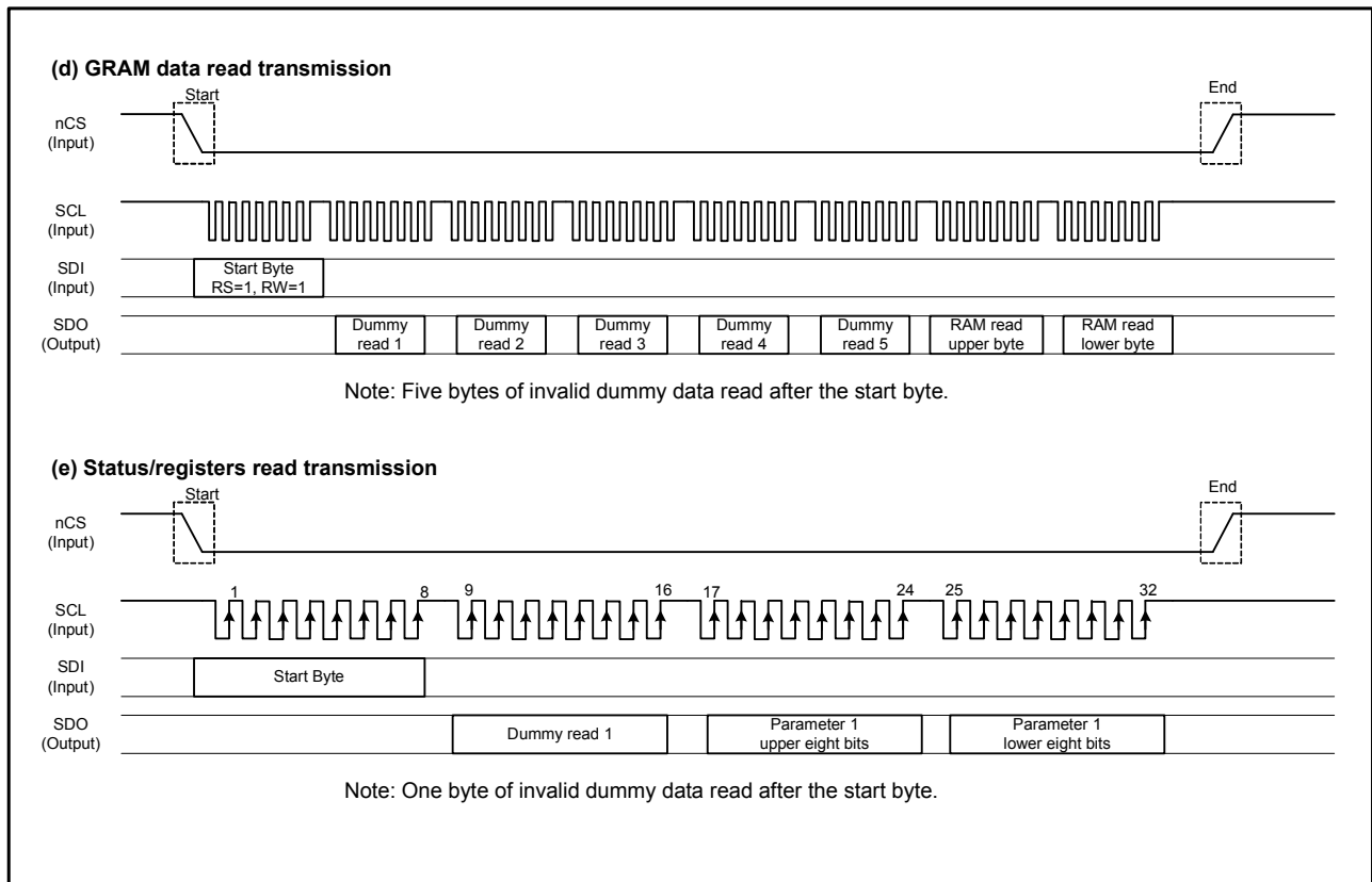
Figure 8 Data transmission through serial peripheral interface (SPI) (2)
