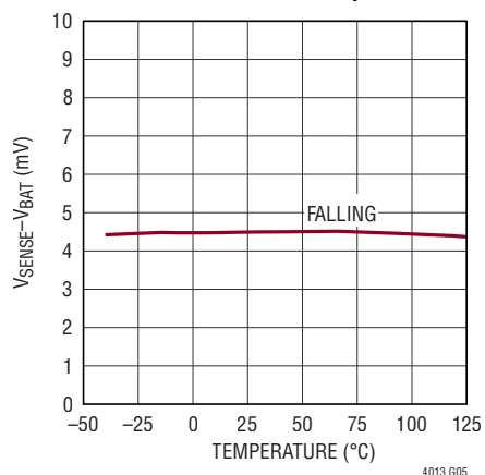
C/10 Thresholds vs Temperature
