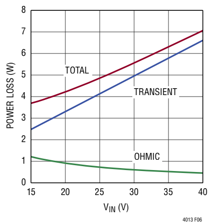
Figure 6. Bottom MOSFET Power Loss Example
