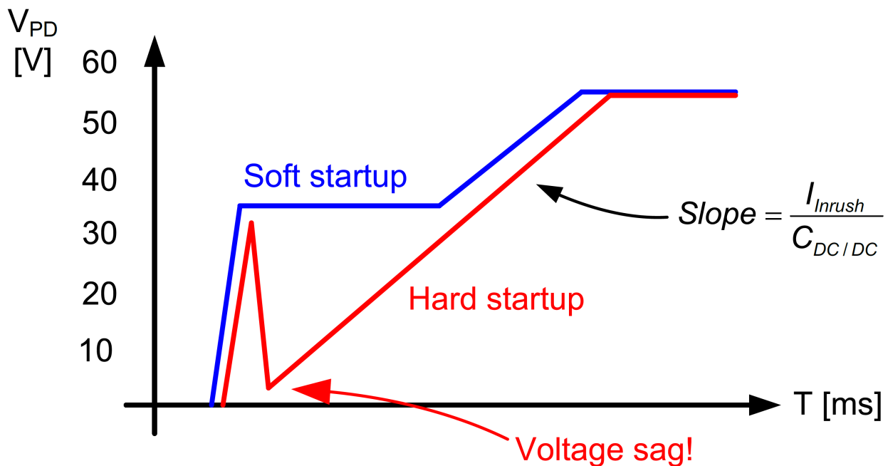
Figure 1-3. Startup Comparison
