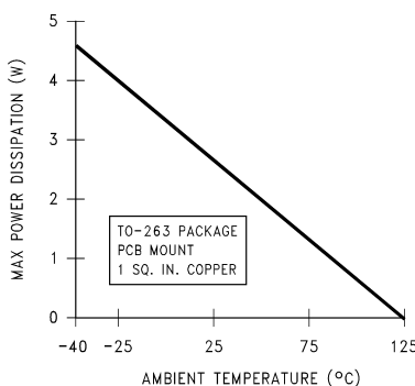
Figure 18. Maximum power dissipation vs ambient temperature for DDPAK/TO-263 package
