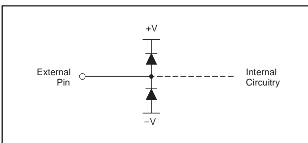
Figure 2. ESD Protection Diodes
