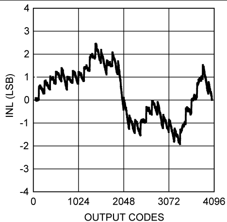
Figure 3. INL at V_A = 3\text{ V}
