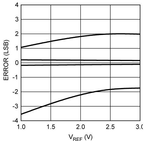
Figure 7. INL/DNL vs V_{\text{REF}} at V_A = 3\text{ V}
