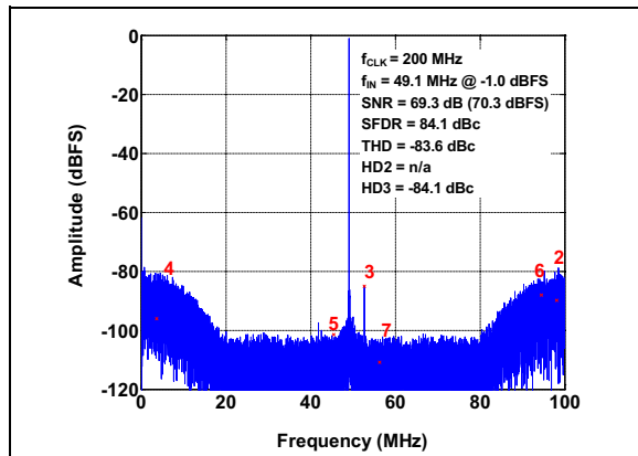
FIGURE 3-8: FFT for 49.1 MHz Input Signal with NSR enabled: NSR = 69, f_S = 200\text{ Mps} , A_{IN} = -1\text{ dBFS} .
