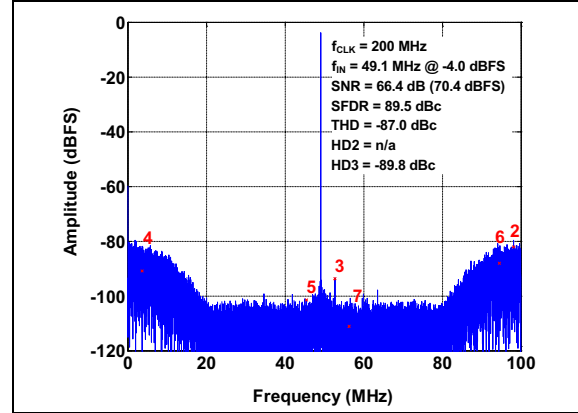
FIGURE 3-11: FFT for 49.1 MHz Input Signal with NSR enabled: NSR = 69, f_S = 200\text{ Mps} , A_{IN} = -4\text{ dBFS} .
