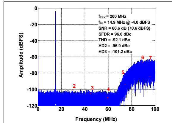
FIGURE 3-10: FFT for 14.9 MHz Input Signal with NSR enabled: NSR = 63, f_S = 200\text{ Mps} , A_{IN} = -4\text{ dBFS} .
