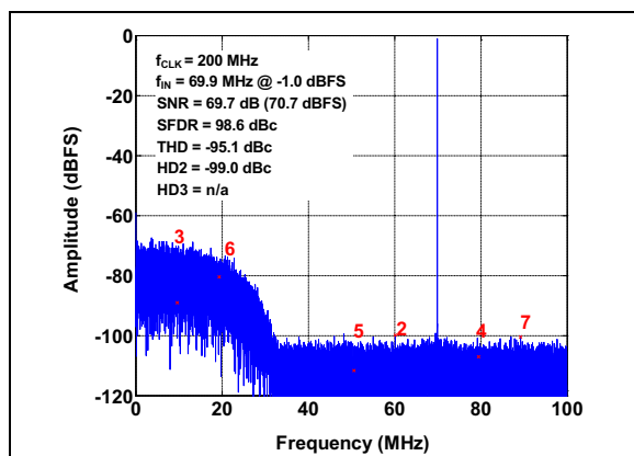
FIGURE 3-9: FFT for 69.9 MHz Input Signal with NSR enabled: NSR = 75, f_S = 200\text{ Mps} , A_{IN} = -1\text{ dBFS} .
