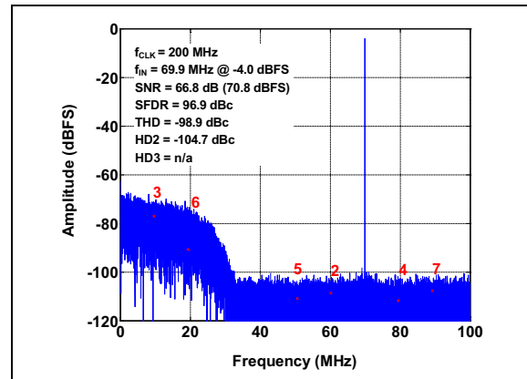
FIGURE 3-12: FFT for 69.9 MHz Input Signal with NSR enabled: NSR = 75, f_S = 200\text{ Mps} , A_{IN} = -4\text{ dBFS} .
