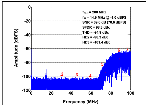
FIGURE 3-7: FFT for 14.9 MHz Input Signal with NSR enabled: NSR = 63, f_S = 200\text{ Mps} , A_{IN} = -1\text{ dBFS} .
