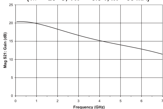
Figure 4: Gain vs. Frequency De-embedded 50 \Omega S-parameter (T A = +25 °C, V CC = +3.8 V, I CC = 33 mA)
