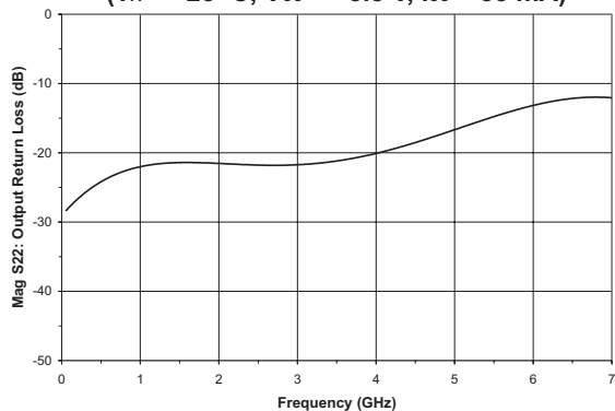
Figure 7: Output Return Loss vs. Frequency De-embedded 50 \Omega S-parameter (T A = +25 °C, V CC = +3.8 V, I CC = 33 mA)
