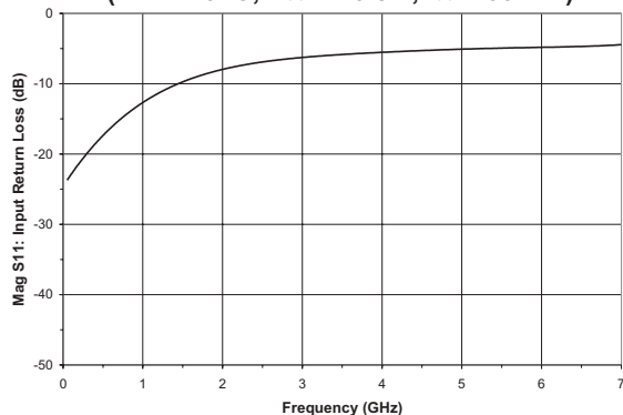
Figure 6: Input Return Loss vs. Frequency De-embedded 50 \Omega S-parameter (T A = +25 °C, V CC = +3.8 V, I CC = 33 mA)
