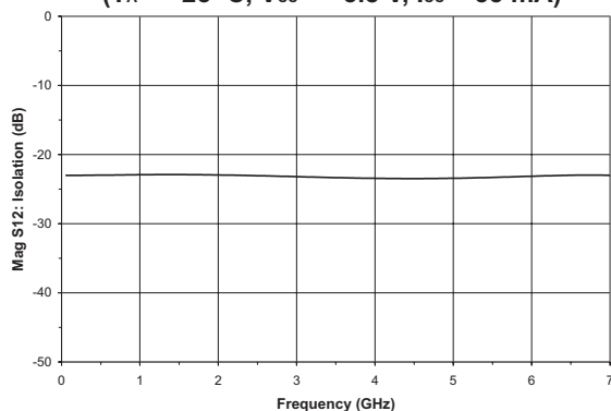
Figure 5: Isolation vs. Frequency De-embedded 50 \Omega S-parameter (T A = +25 °C, V CC = +3.8 V, I CC = 33 mA)
