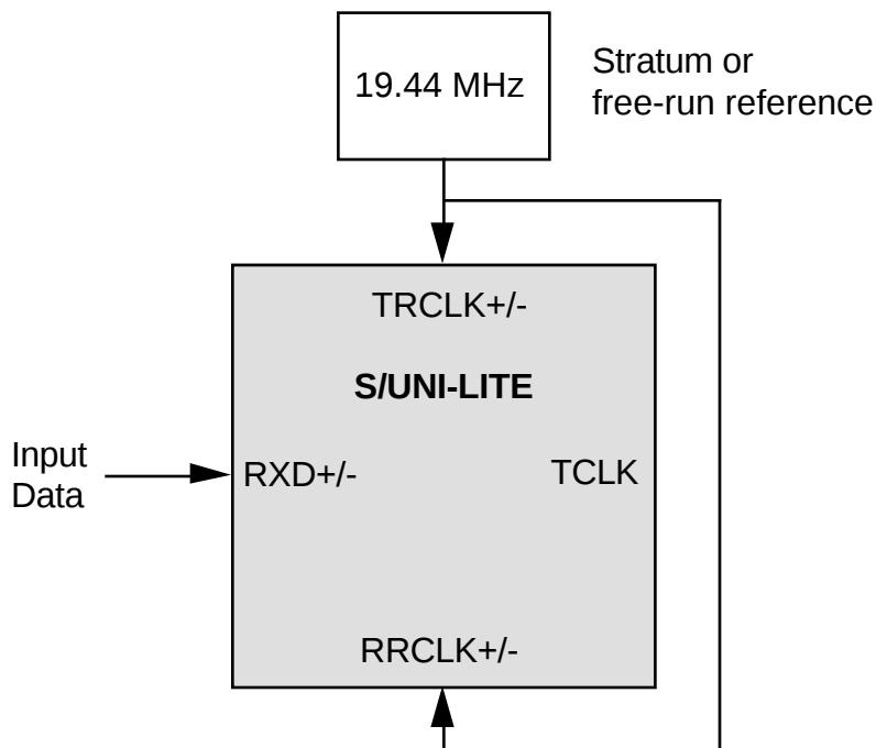
Fig. 17a Mode A: Clock Synthesis
