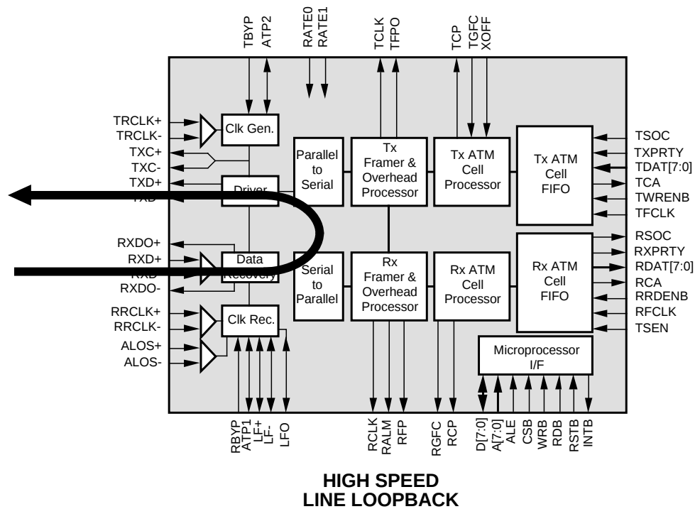
Fig. 11 Loopback Operation
