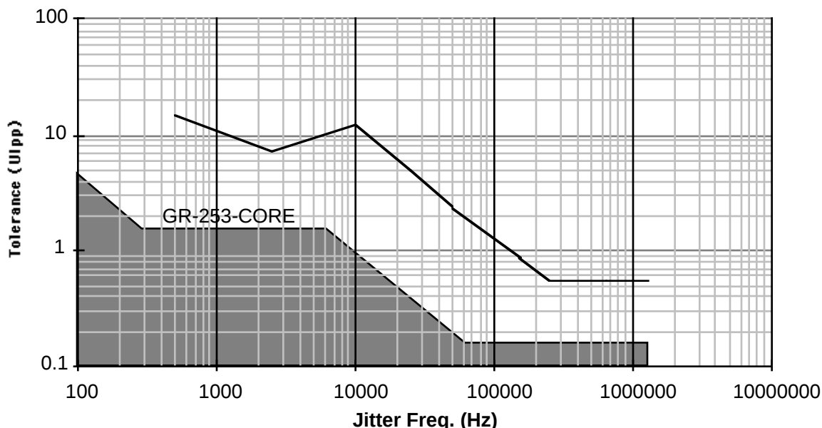
Fig. 2 STS-3c/STM-1Jitter Tolerance
