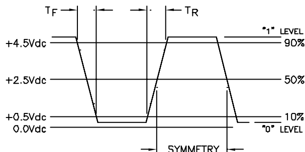
OUTPUT WAVEFORM
