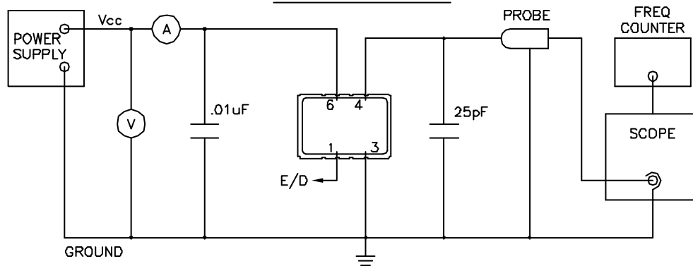
TEST CIRCUIT
