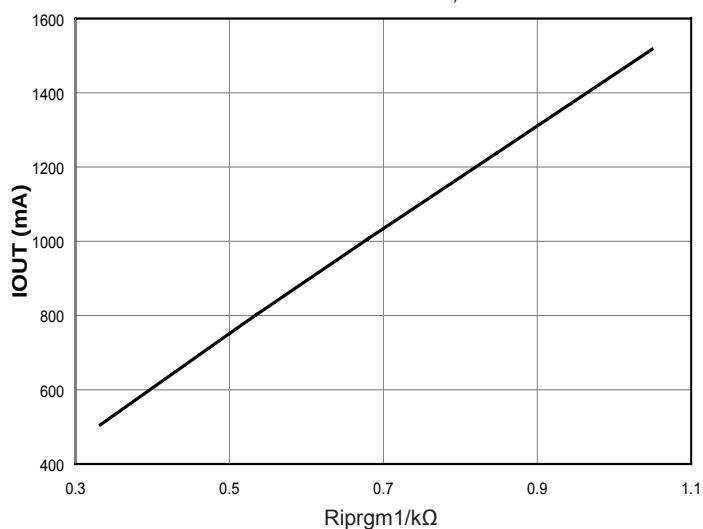
IOUT vs. IPRGM Resistance, T = +25 °C
