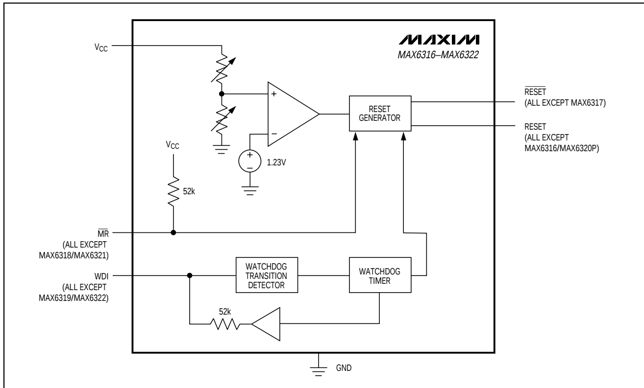
Figure 1. Functional Diagram
