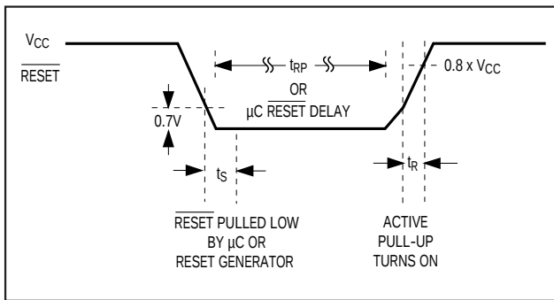
Figure 5. Bidirectional \overline{\text{RESET}} Timing Diagram
