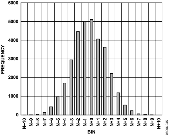
Figure 39 105 MSPS, Grounded Input Histogram
