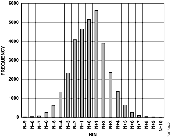
Figure 38. 80 MSPS, Grounded Input Histogram
