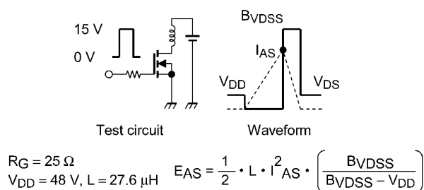
Fig. 8.15 Test Circuit/Waveform
